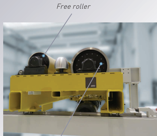
Driven roller
